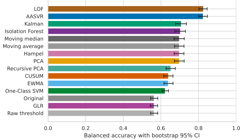
Figure 6: Bootstrap uncertainty for held-out hydroponic synthetic-fault balanced accuracy. Intervals are computed by resampling injected-fault trials. The result should be read together with the paired tests because AASVR and LOF are close on point-wise balanced accuracy, while false-actuation behavior differs strongly.
